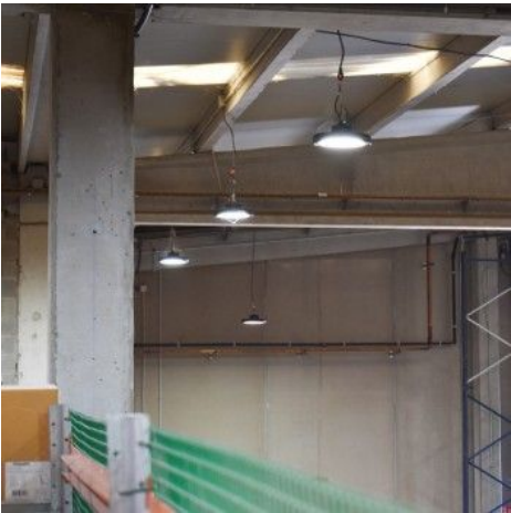
Industrial LED High Bay light with motion sensor - 150W - Philips driver - Dimmable 1-10V - IP65
