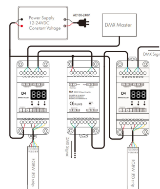
Wiring Diagram
