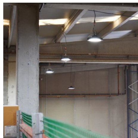
Industrial LED High Bay light with motion sensor - 200W - Philips driver - Dimmable 1-10V - IP65
