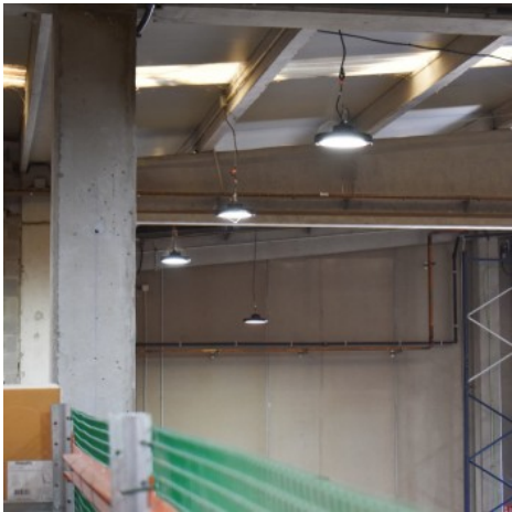
Industrial LED High Bay - LIFUD Driver - 150W - 160lm/W - PHILIPS Chip - Dimmable 1-10V - IP65
