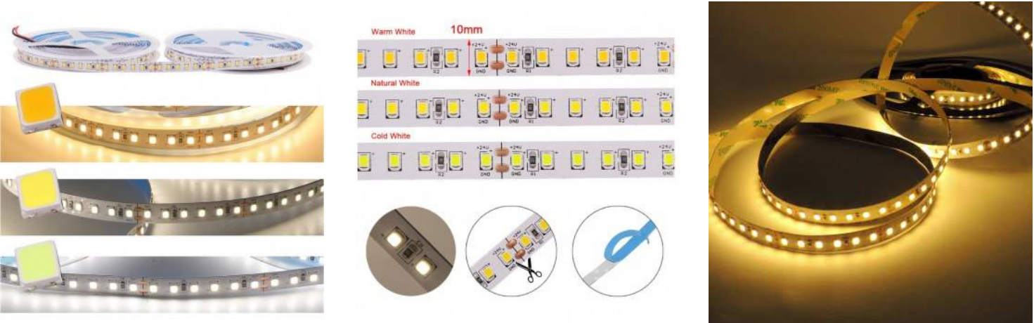
LED Strip 24V DC - 18W/m - Single Color - 10mm - IP20 - Roll 5 meters - 120ch/m
